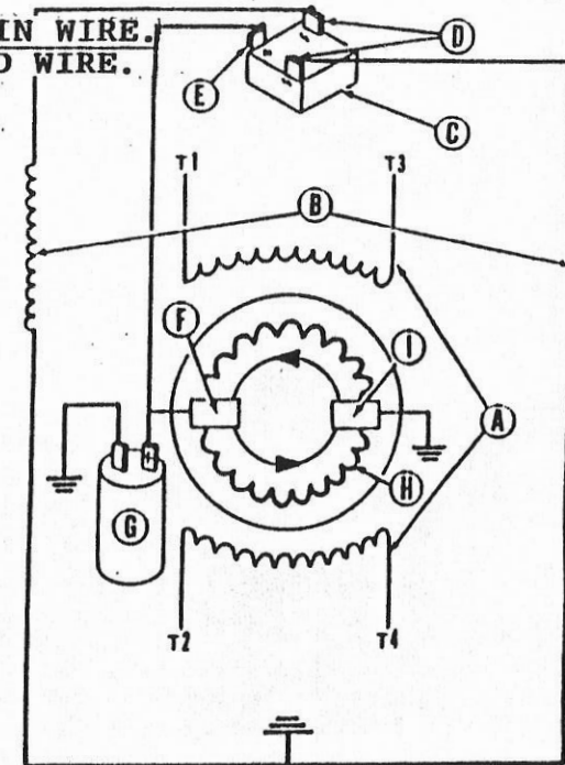
— View of basic generator circuitry.
