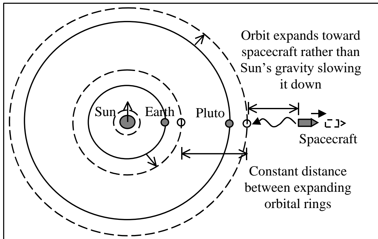
Figure 13 (3-26) Expanding solar system differs from Newtonian gravity
