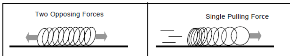
Figure 27 Two opposing forces, stretching a spring horizontally, compared to a single pulling force
